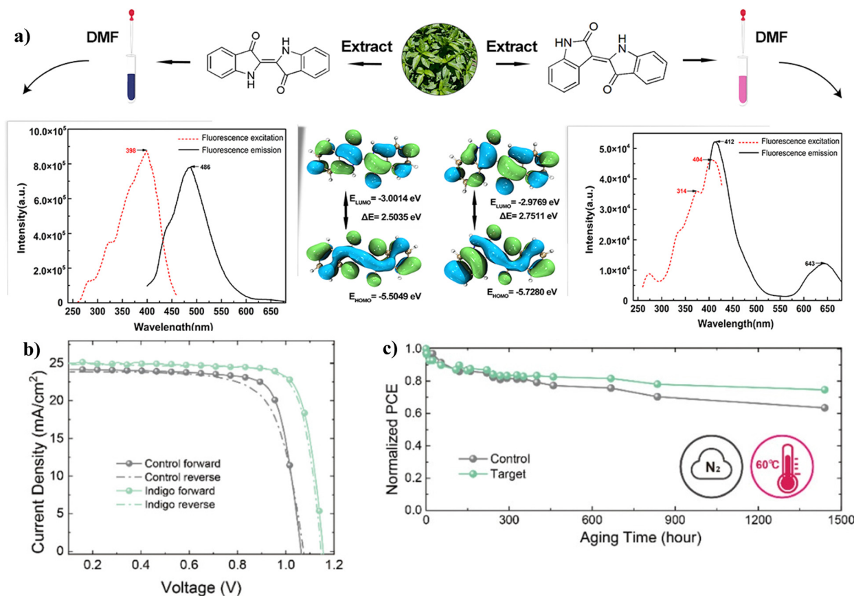
Fig. 14 (a) Structures of indigo (left) and its oxidized derivative indirubin (right), 141 (b) J – V curves for PSCs with and without indigo. (c) Normalized PCE for PSCs with and without indigo; reproduced from ref. 142 with permission from Wiley-VCH GmbH (2022).
