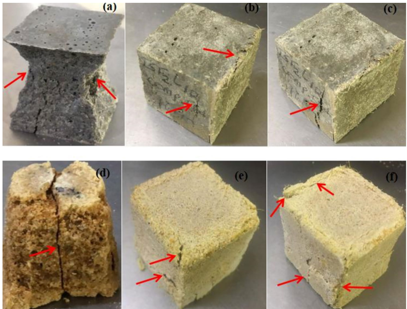
Fig. 18. The residual after compressive strength test at 56 days (a) control mixture, (b) sisal fiber reinforced, (c) second residual of (b), (d) the residual cured in 5% HCl for 56 days, (e) sisal fiber reinforced residual cured in 5% HCl, and (f) the second residual of (e) respectively.
