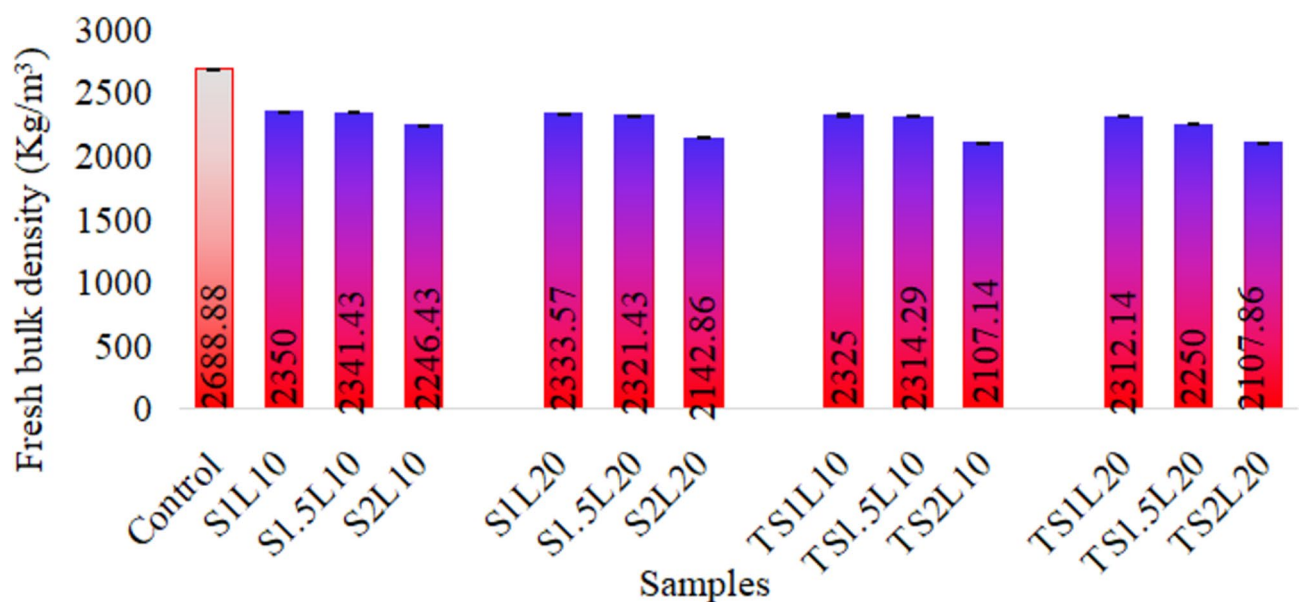
Fig. 7. The fresh density of mortar reinforced by treated and raw sisal fibers.
