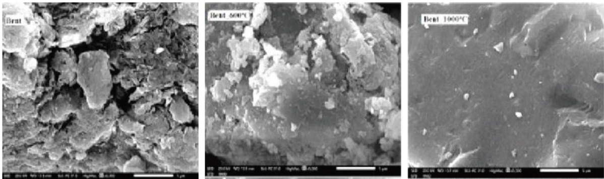
FIGURE 11: Microstructure of raw and activated bentonite by El Refaey [60].
