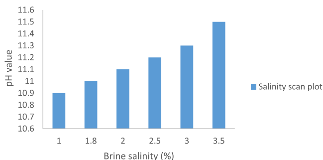
Figure 7. Plot showing alkalinity as a function of salinity.
