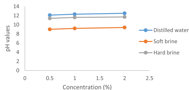
Figure 4. pH Values of OME.
