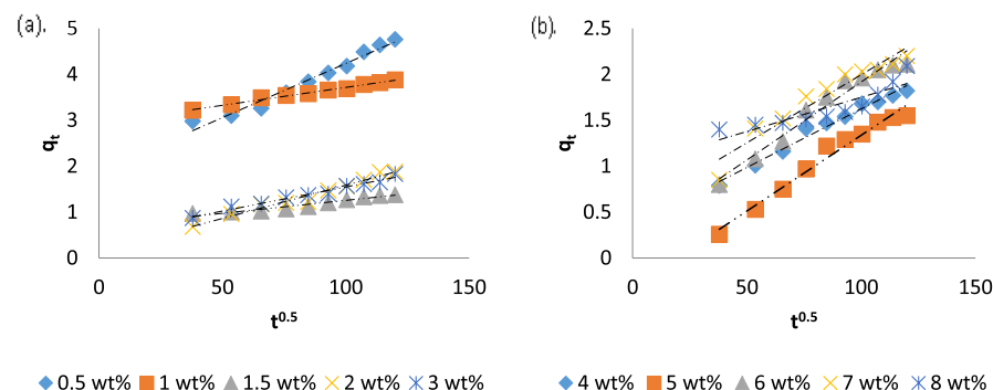
Figure 19. Intraparticle diffusion kinetic model for (a) 0.5–3 wt % surfactant conc. (b) 4–8 wt % surfactant conc.
