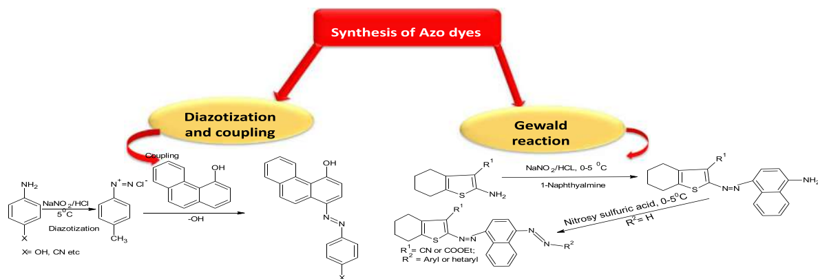
Fig. 2. Synthesis of azo dyes.
