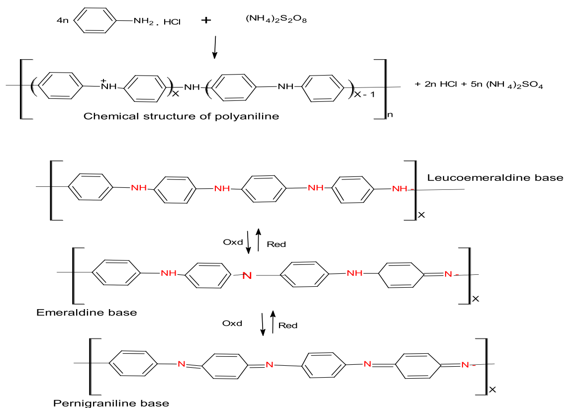
Fig. 7. Oxidative polymerization of polyaniline into chemical forms.
