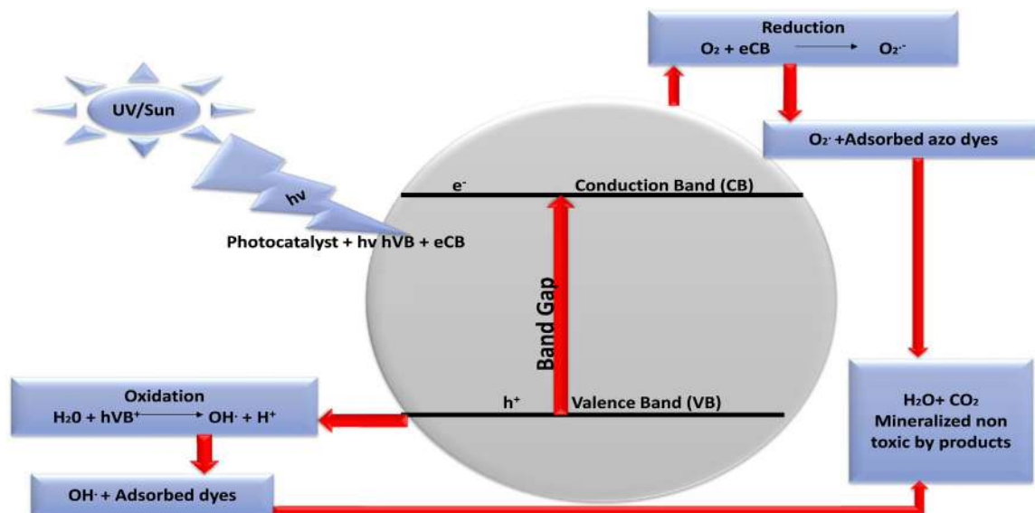
Fig. 6. Mechanism of Azo dye degradation in photocatalysis.
