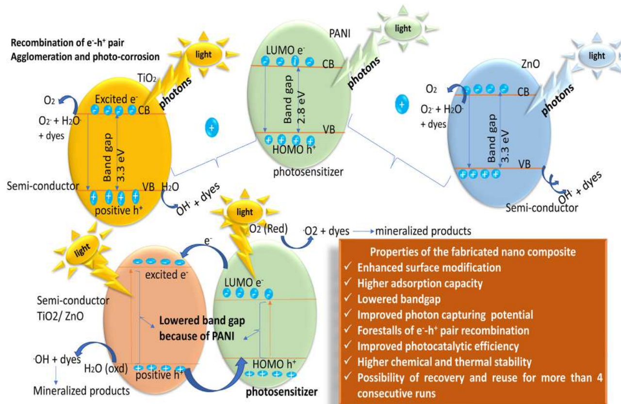
Fig. 9. Mechanism of dye interaction with pure semiconductors and PANI/TiO 2 nanocomposite.
