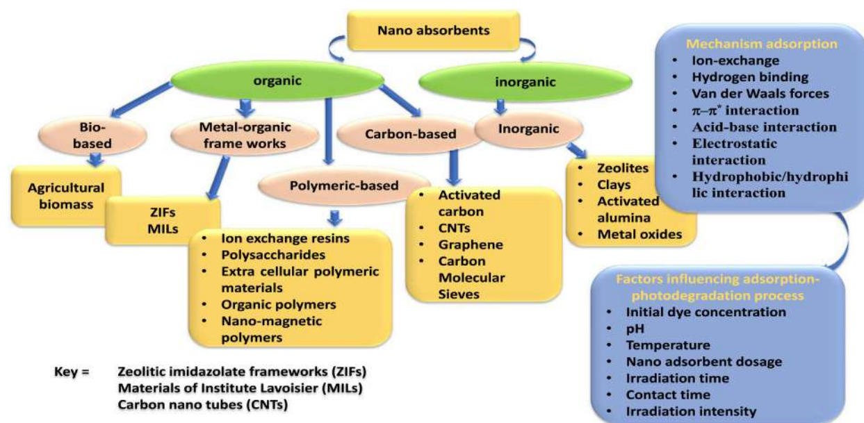
Fig. 5. Categories of nano-adsorbent, mechanism and parameters influencing their performance.
