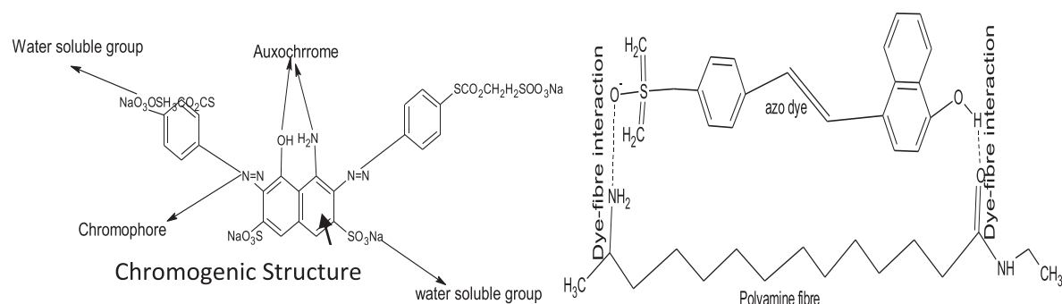
Fig. 3. a: Structure of reactive azo dye. b: Structure of Dye-fibre.
