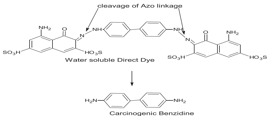
Fig. 4. Bond cleavage of azo dye in textile wastewater.
